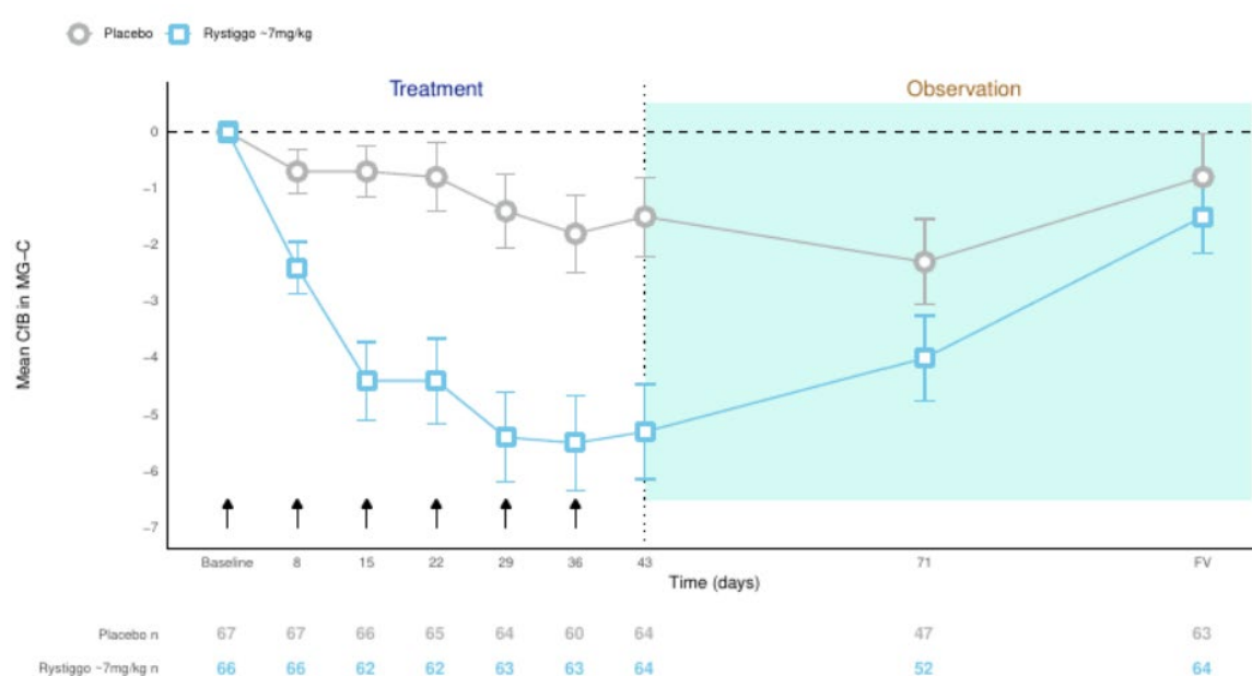
Figure 2: Observed mean change from Baseline in MG-C score (Study MG0003)
